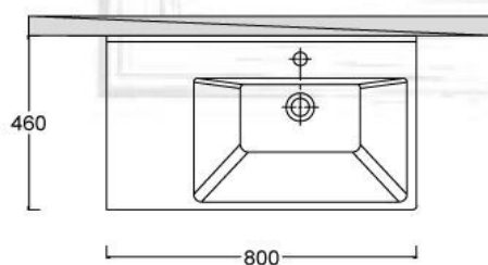
RAKAN 80 FRONT ELEVATION
