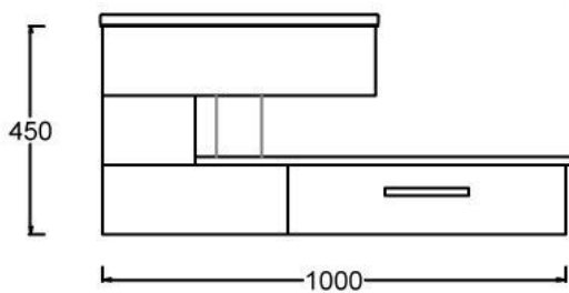
LEU 100 FRONT ELEVATION
